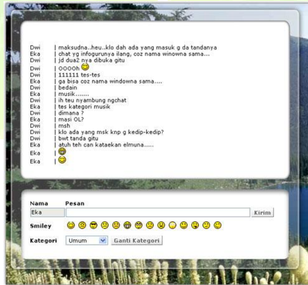
Gambar 22. Menu Chatting
